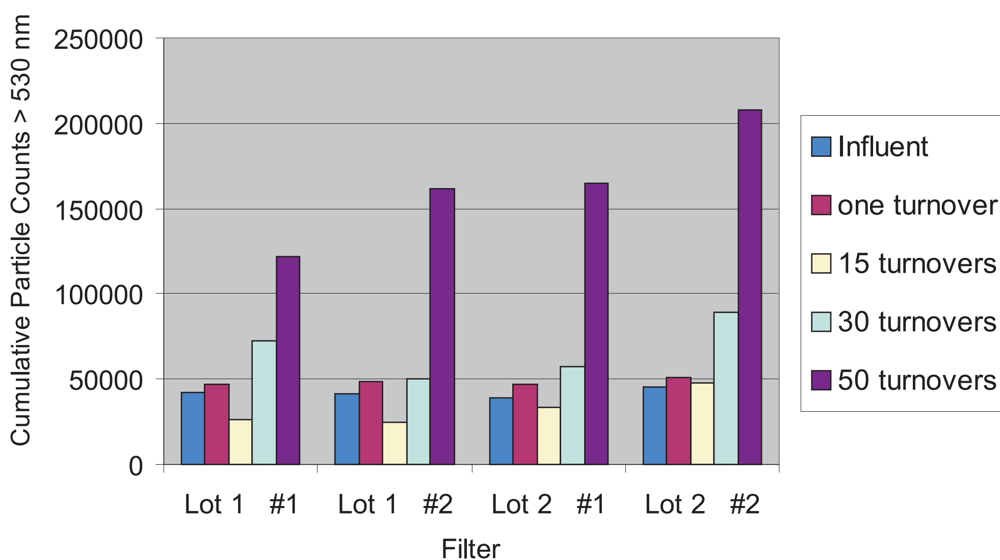
Fumed Silica Slurry Filtration with Peristaltic Pump
