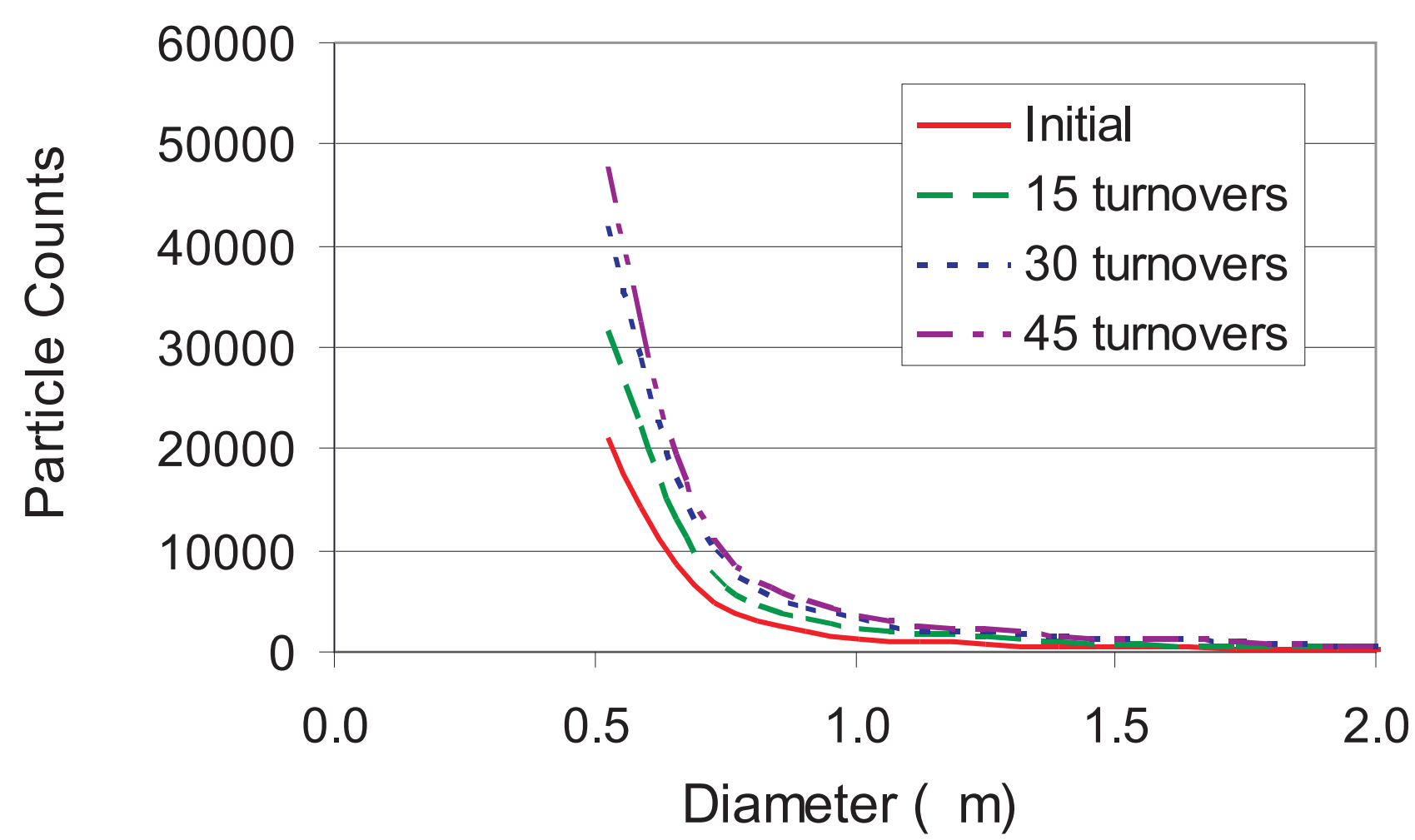
PSD summary for Rotary Peristaltic Pump
