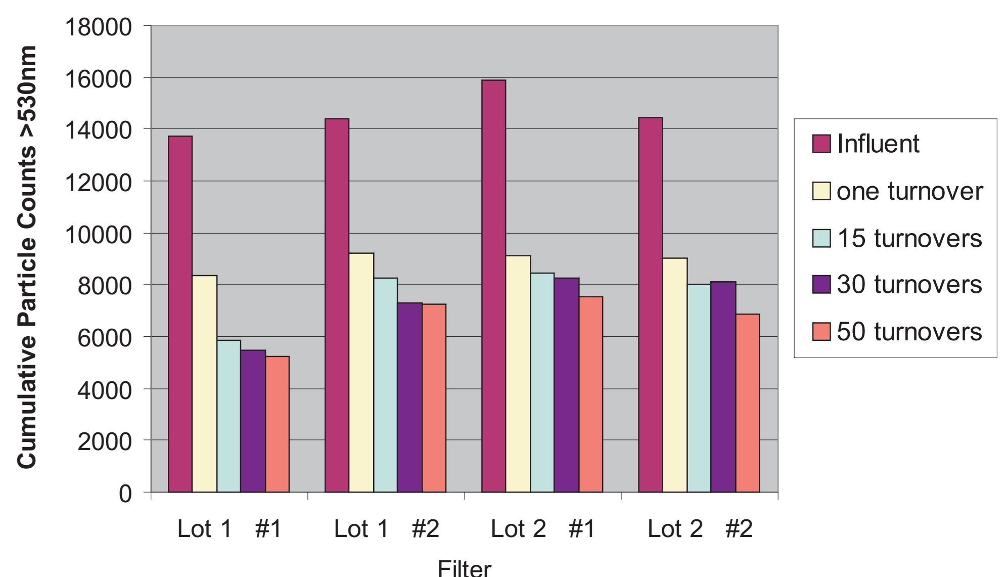
Fumed Silica Slurry Filtration with Levitronix Pump
