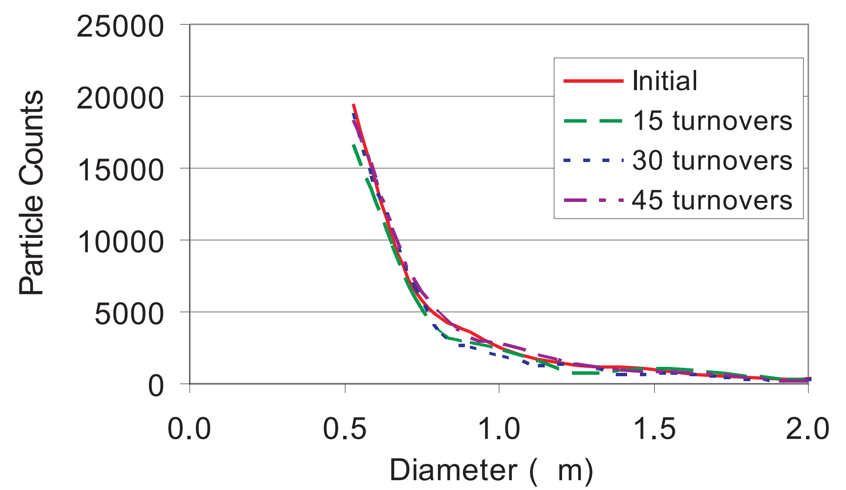
PSD summary for Levitronix BPS-1
