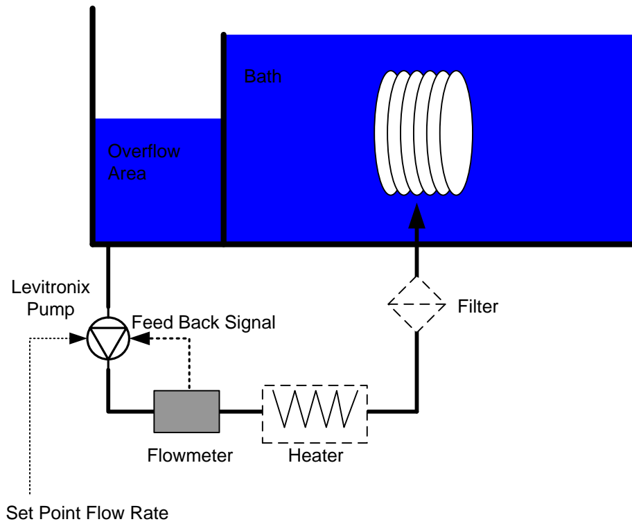
Figure 1: System Overview of the Closed-Loop Flow Control System
